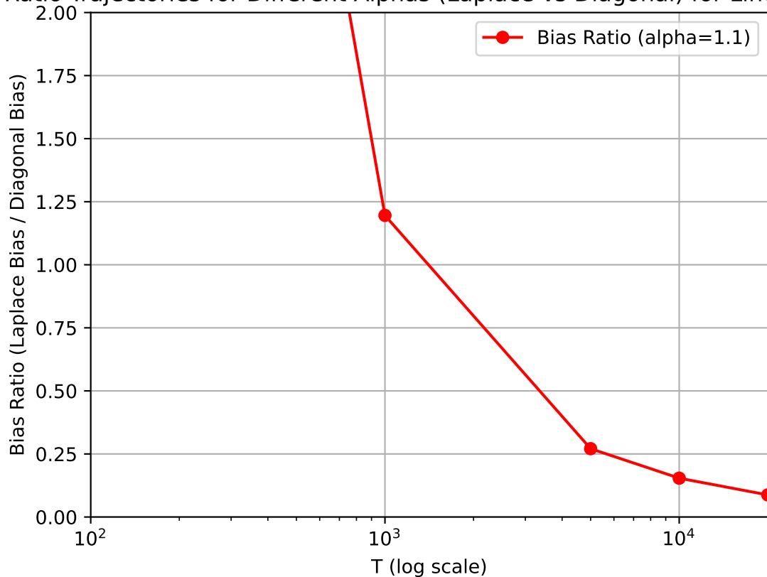
Bias Ratio Trajectories for Different Alphas (Laplace vs Diagonal) for Linear sche
