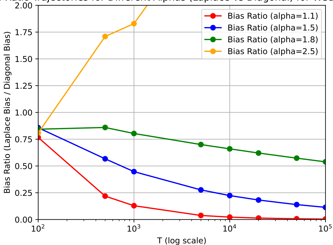
Bias Ratio Trajectories for Different Alphas (Laplace vs Diagonal) for WSD scheme
