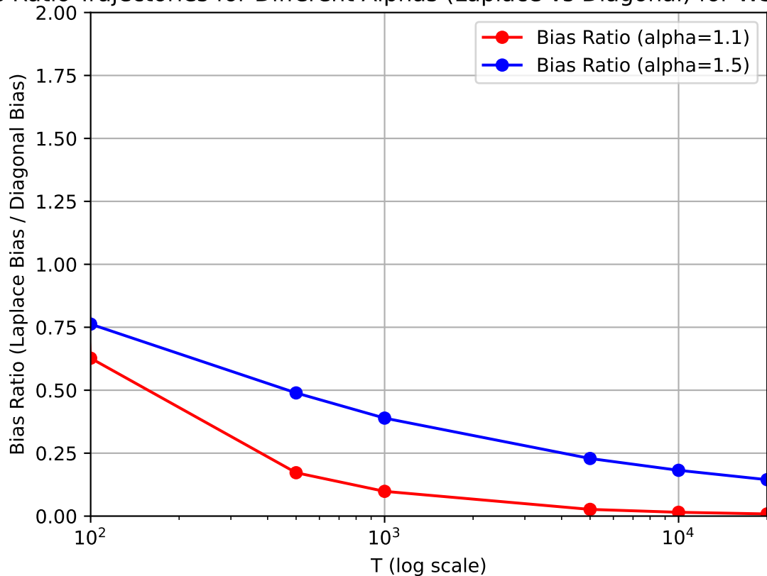
Bias Ratio Trajectories for Different Alphas (Laplace vs Diagonal) for WSD sche
