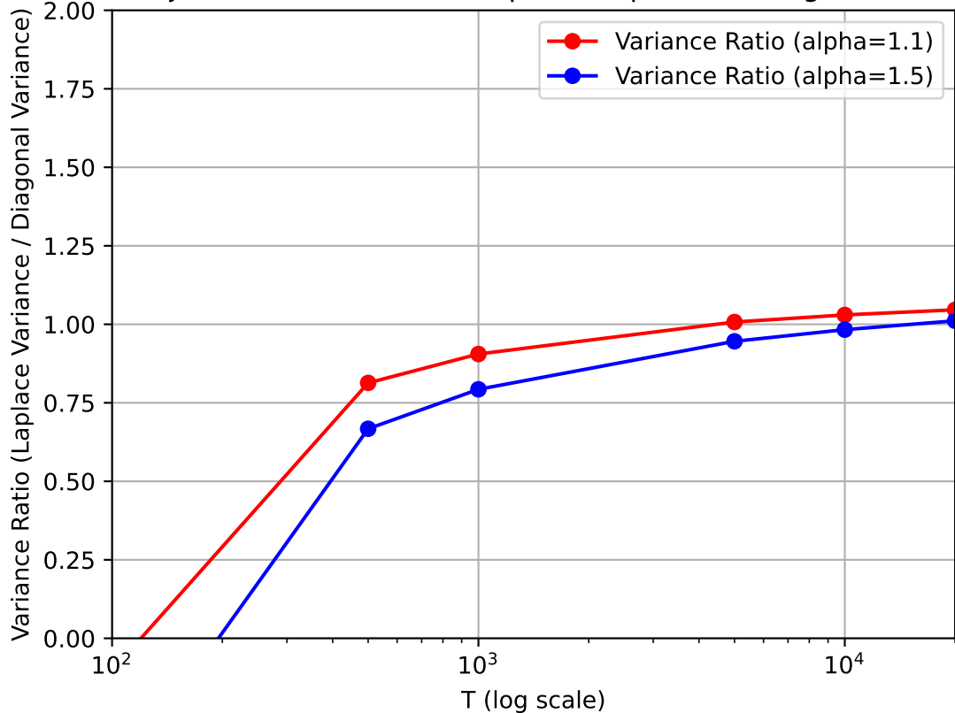
Variance Ratio Trajectories for Different Alphas (Laplace vs Diagonal) for WSD sch
