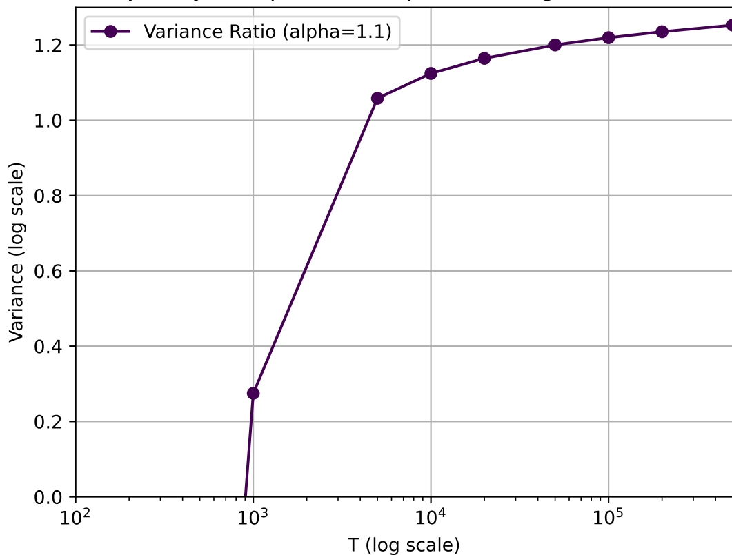
Variance Trajectory for \alpha=1.1 (Laplace vs Diagonal) for WSD schedule
