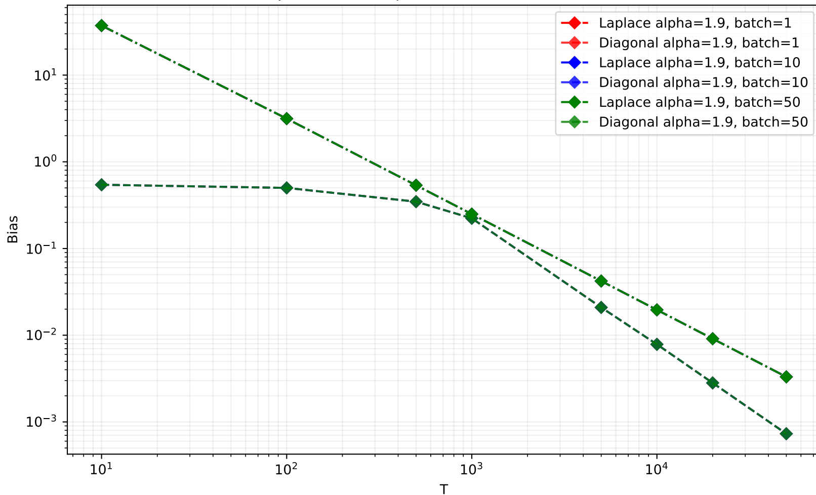
Bias trajectories for \alpha=1.9 and different batch sizes
