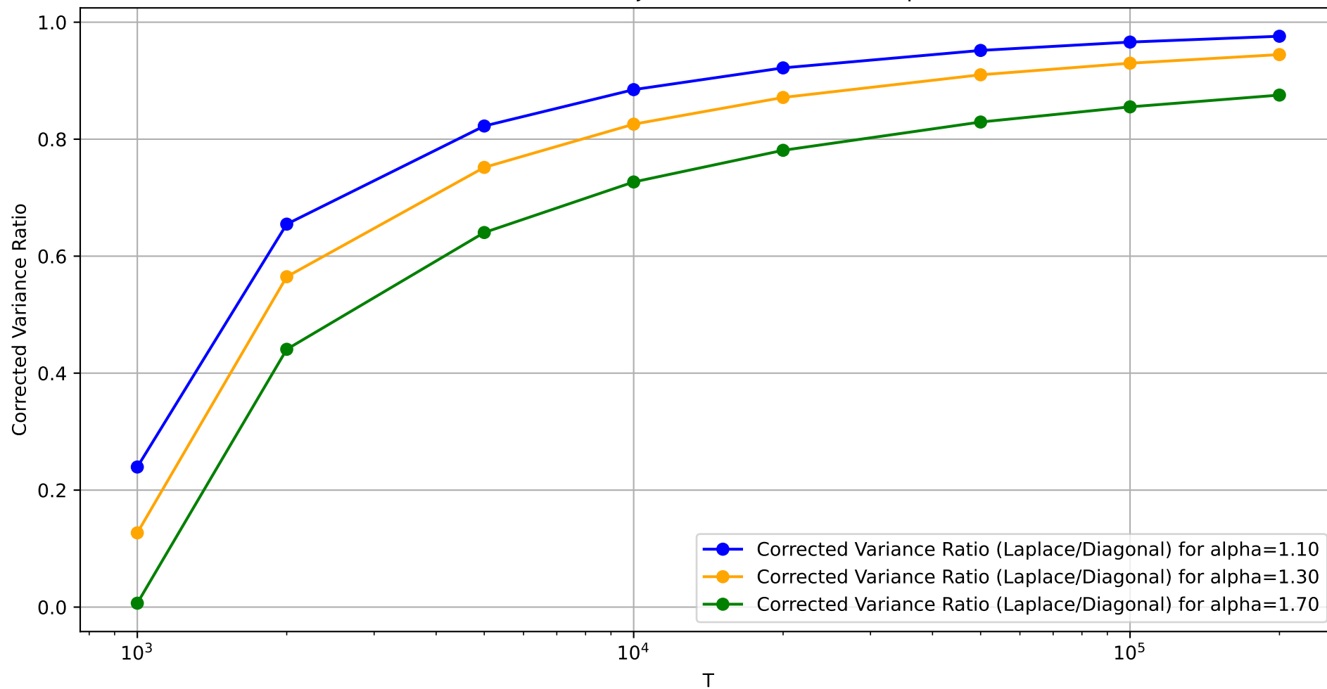
Corrected Variance Ratio Trajectories for Different Alphas, dim=0.02T
