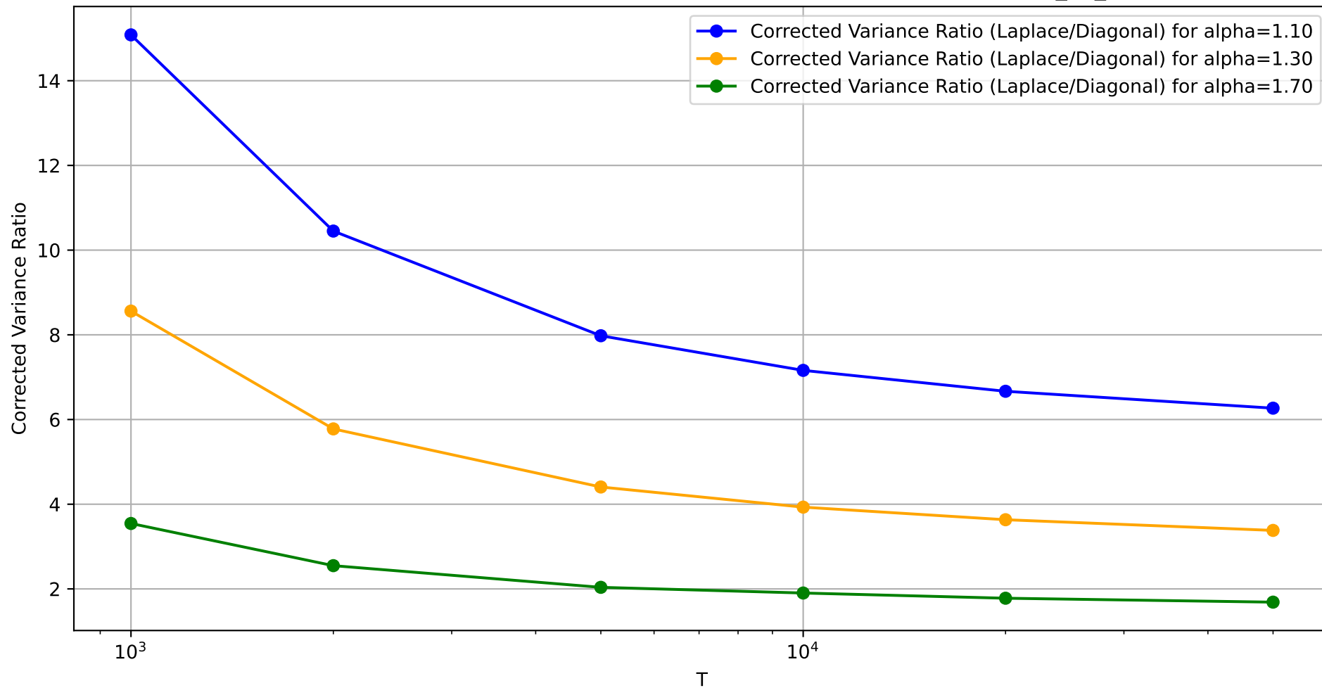
Corrected Variance Ratio Trajectories for Different Alphas, dim=0.05T**1_by_alpha
