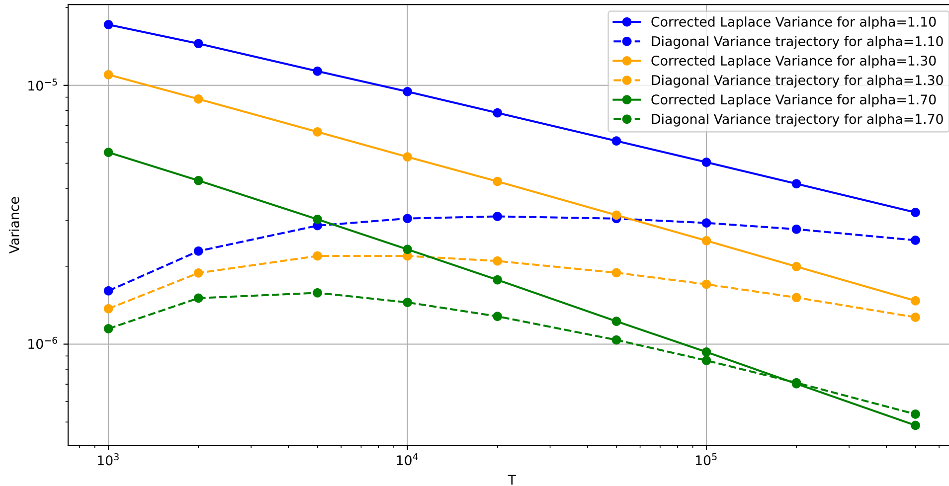
Corrected Variance Trajectories for Different Alphas, (T)^{*(1b(\alpha p1))}
