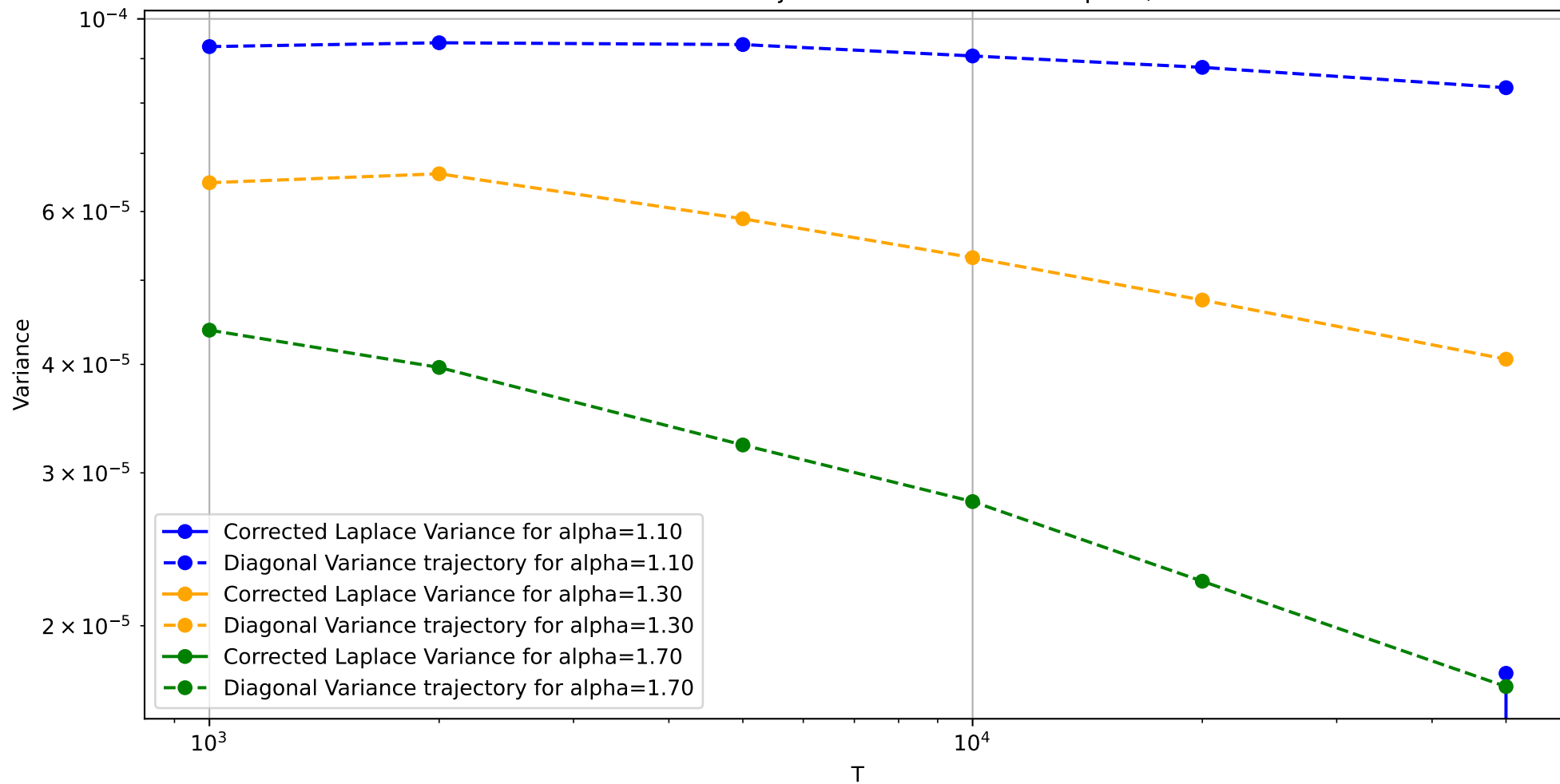
Corrected Variance Trajectories for Different Alphas, 1000
