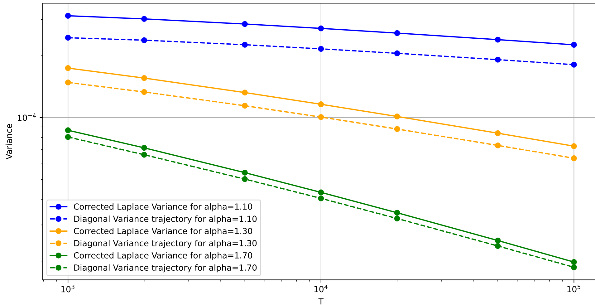
T^{1/2} * \text{Variance Trajectories for Different Alphas, } T b 10^{1/\alpha}
