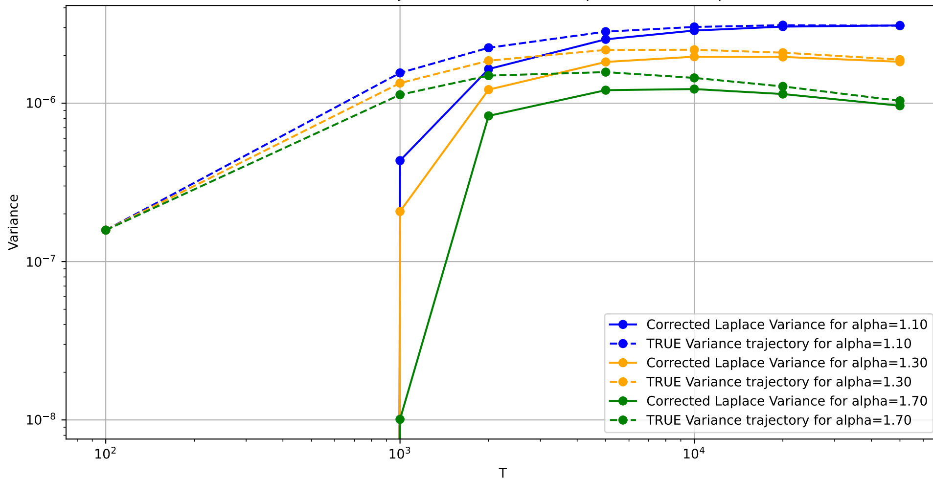
Corrected Variance Trajectories for Different Alphas, Ts50**1balpha+0.2
