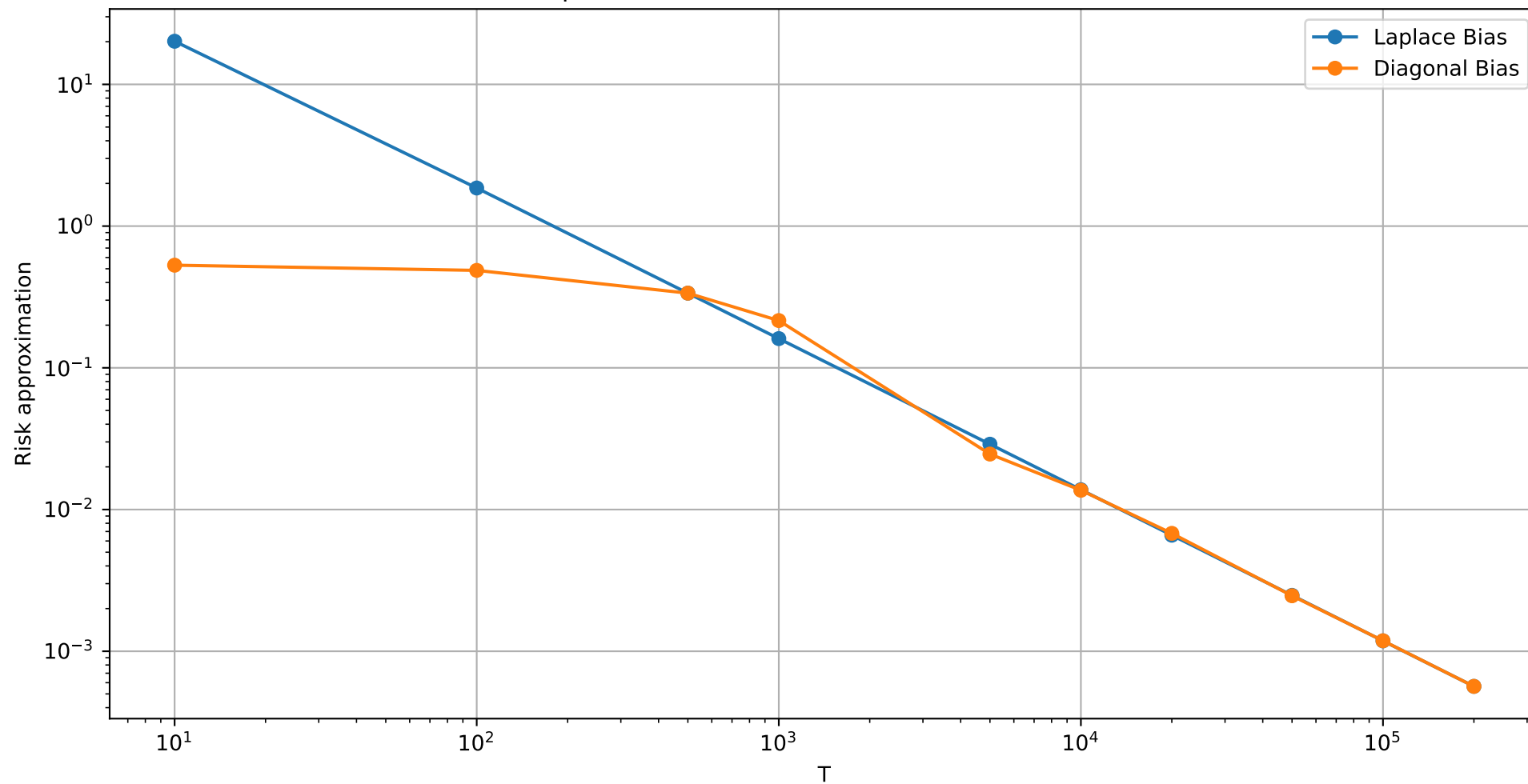
Bias components of Laplace approximation vs Diagonal approximation for linear schedule \alpha=3 , \beta=1.2 , T_{\max}=200000 , K=t/T=1
