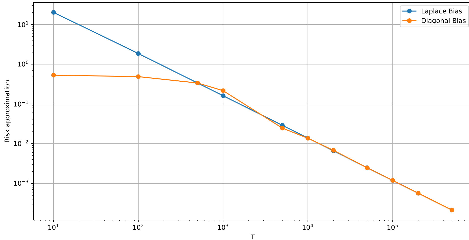
Bias components of Laplace approximation vs Diagonal approximation for linear schedule \alpha=3 , \beta=1.2 , T_{\max}=500000 , K=t/T=1
