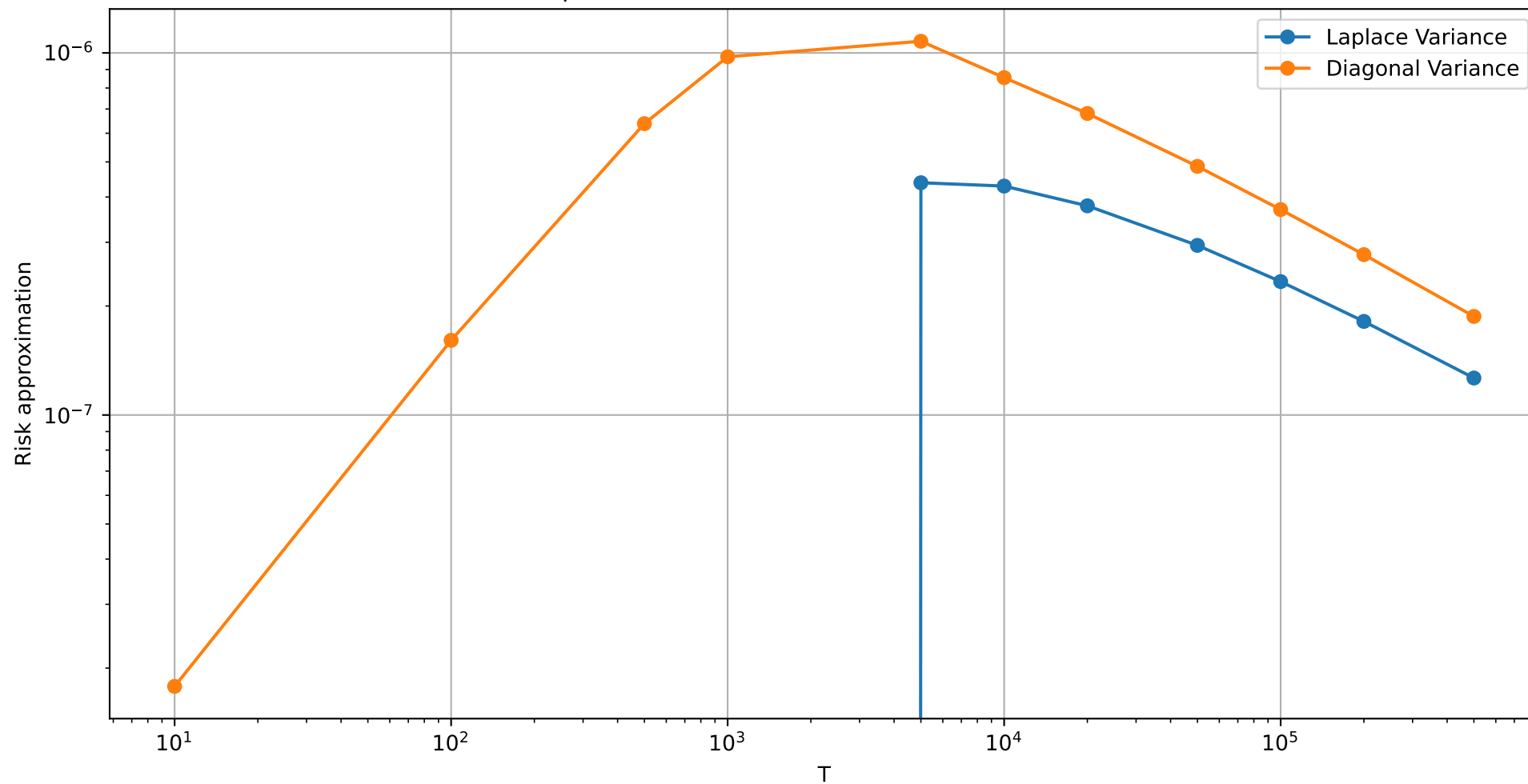
Variance components of Laplace approximation vs Diagonal approximation for linear schedule \alpha=3 , \beta=1.2 , T_{\max}=500000 , K=t/T=1
