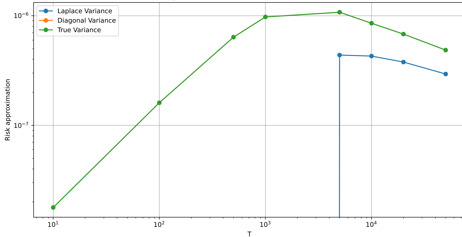
Variance components of Laplace approximation vs Diagonal approximation for linear schedule \alpha=3 , \beta=1.2 , T_{\max}=50000 , K=t/T=1
