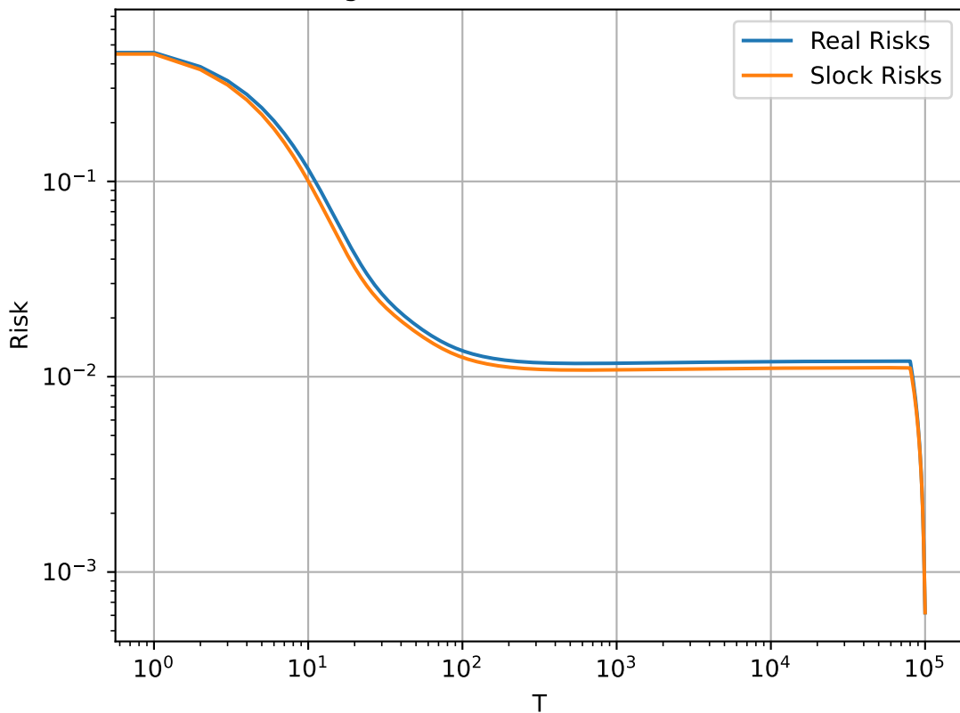
Comparison of Real Risks and Slock Risks for SGD with WSD schedule \sigma=0.5 , \beta=2 , T=100000
