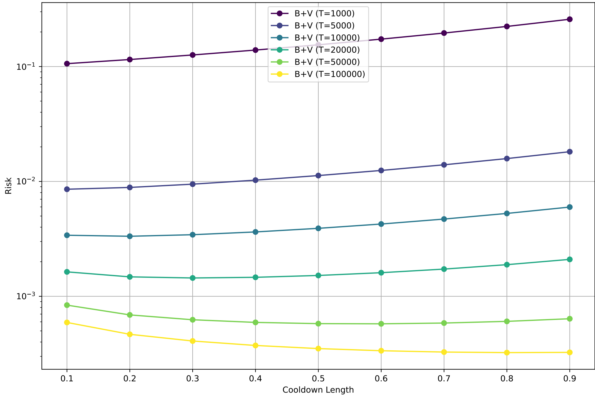
Risk for Different cooldown lengths (SLOCK vs Diagonal) eta=0.001, alpha=1.5
