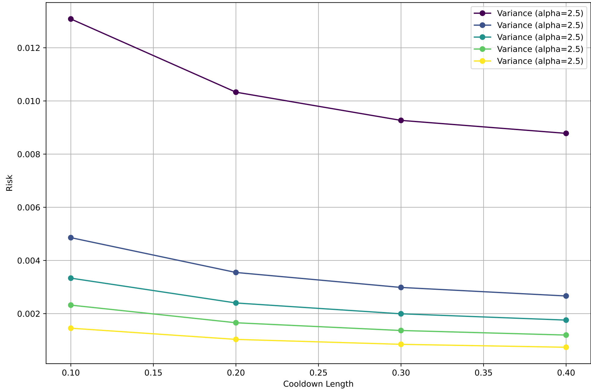
Risk for Different cooldown lengths (SLOCK vs Diagonal) eta=0.01, alpha=2.5
