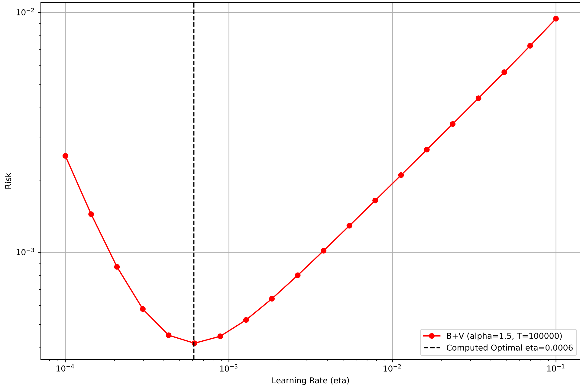
Risk for Different Learning Rates (SLOCK vs Diagonal) \alpha=1.5 , T=100000
