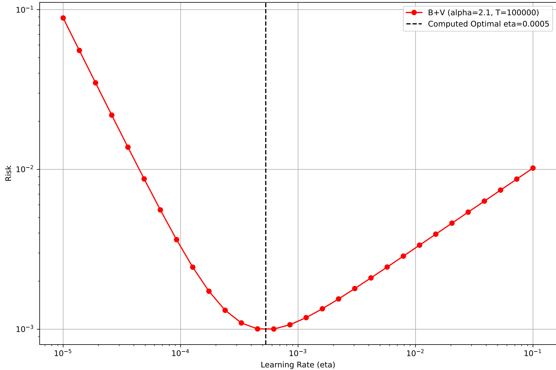
Risk for Different Learning Rates (True vs Approx) \alpha=2.1 , T=100000
