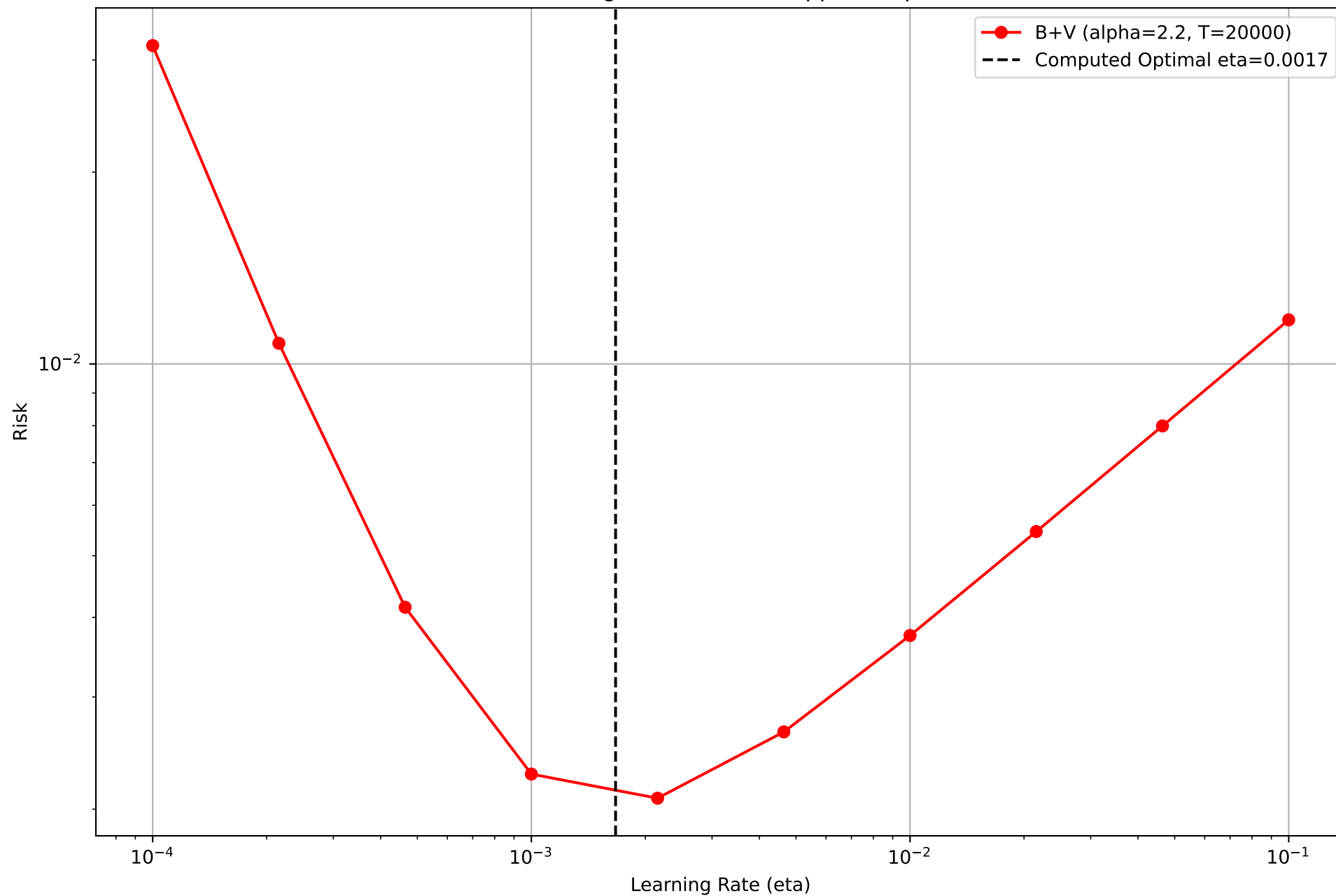
Risk for Different Learning Rates (True vs Approx) \alpha=2.2 , T=20000
