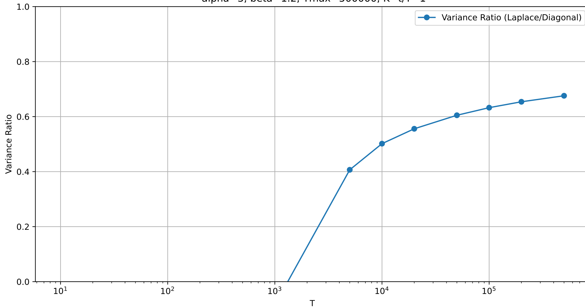
Variance Ratio of Laplace approximation to Diagonal approximation for linear schedule \alpha=3 , \beta=1.2 , T_{\max}=500000 , K=t/T=1
