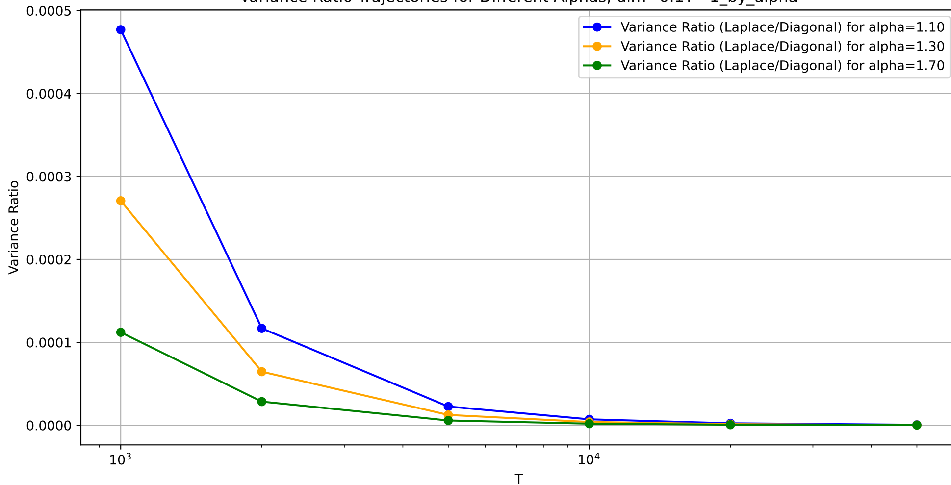
Variance Ratio Trajectories for Different Alphas, \text{dim}=0.1T^{**1\_by\_alpha}
