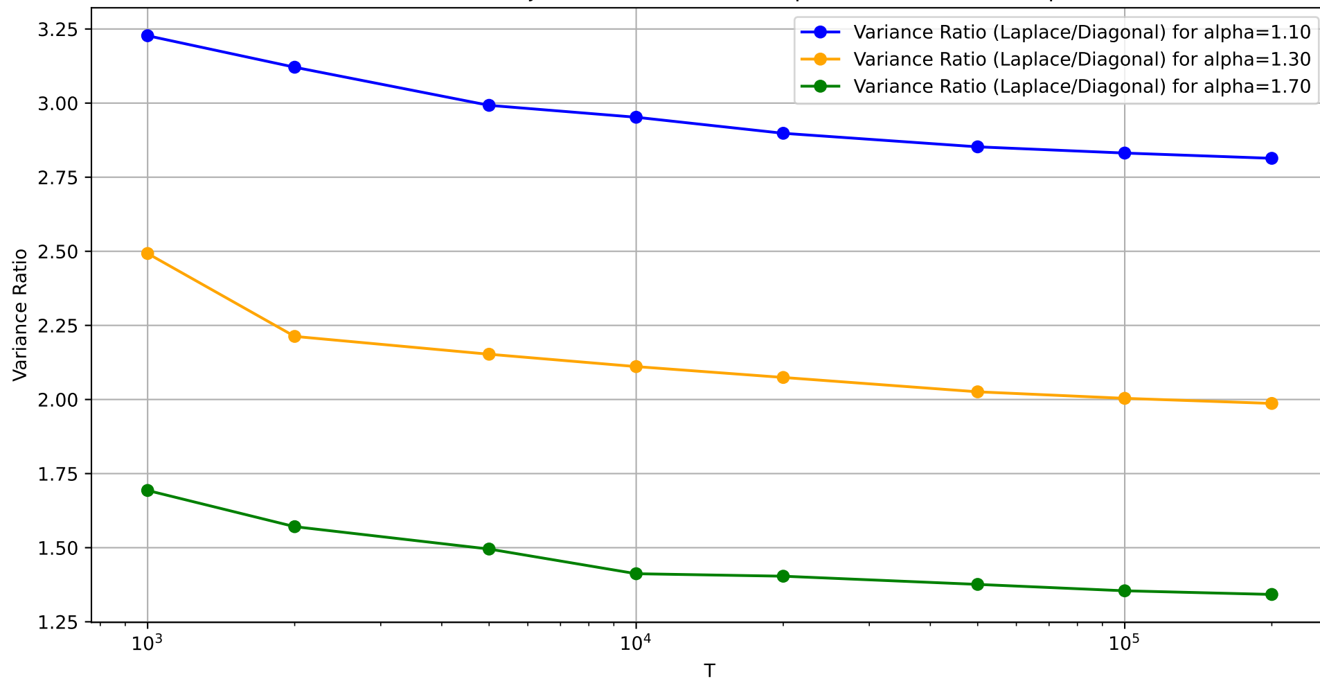
Variance Ratio Trajectories for Different Alphas, dim=Tb10**1balpha
