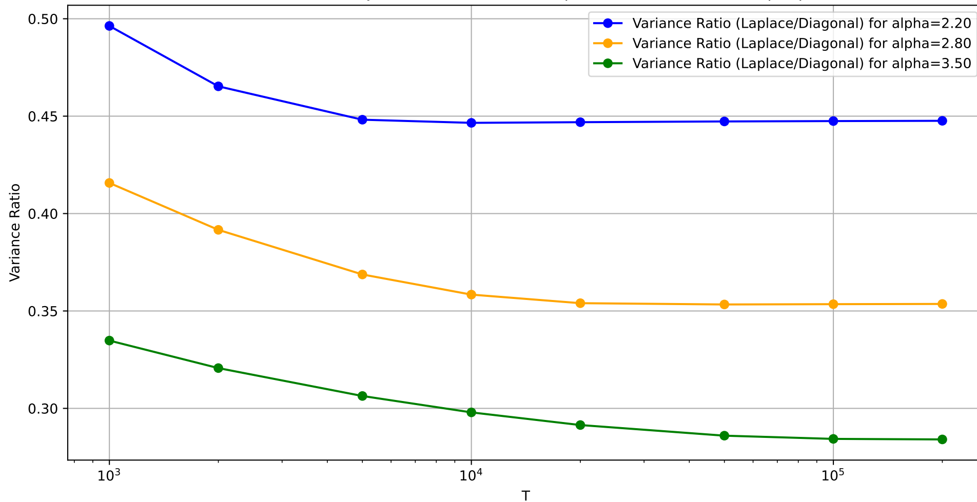
Variance Ratio Trajectories for Different Alphas, \text{dim}=(10T)^{(1b(\text{alphap1}))}
