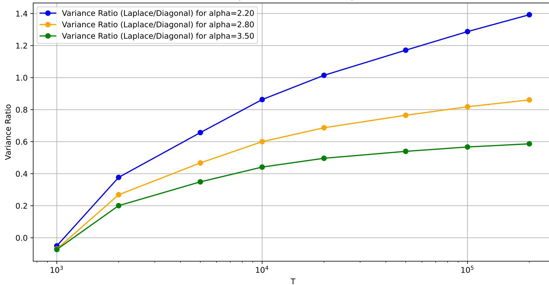
Variance Ratio Trajectories for Different Alphas, dim=0.01T
