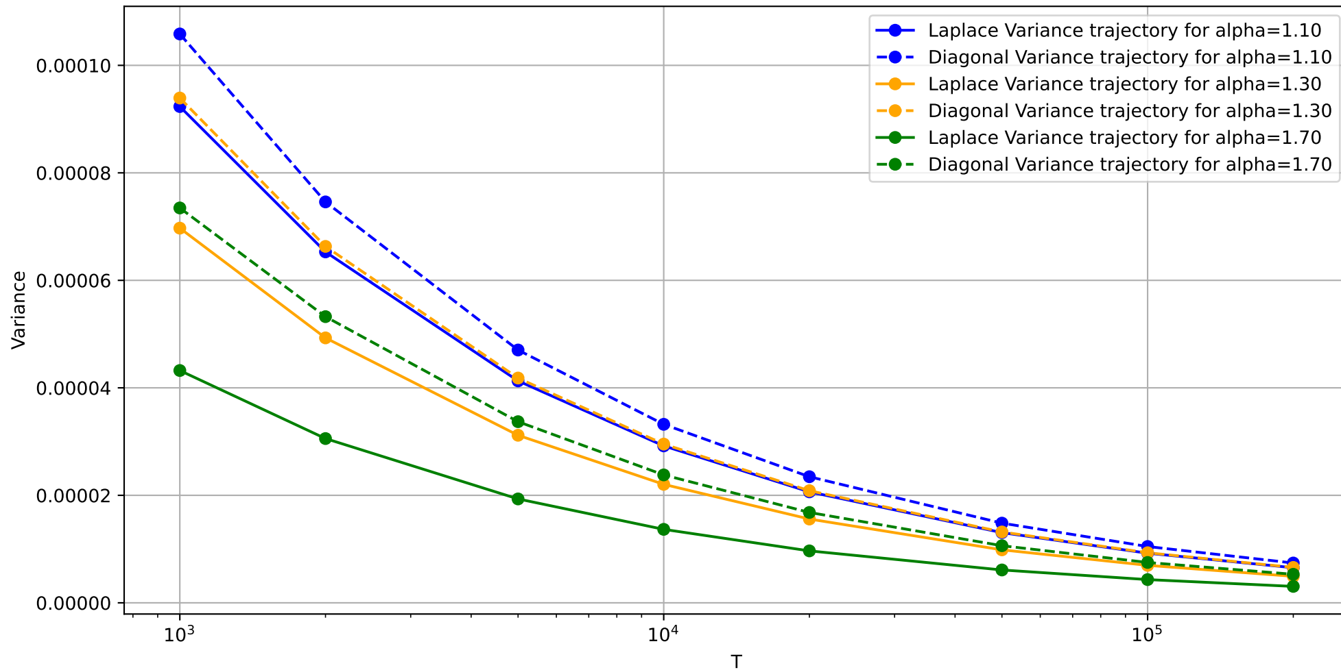
Variance Trajectories for Different Alphas, 10
