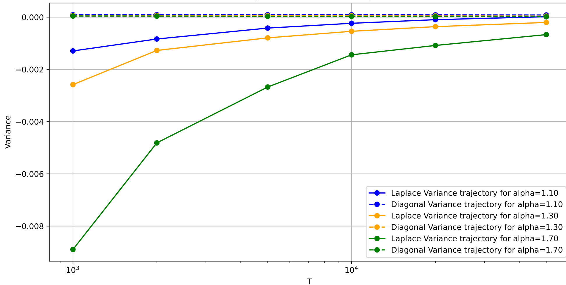
Variance Trajectories for Different Alphas, 1000
