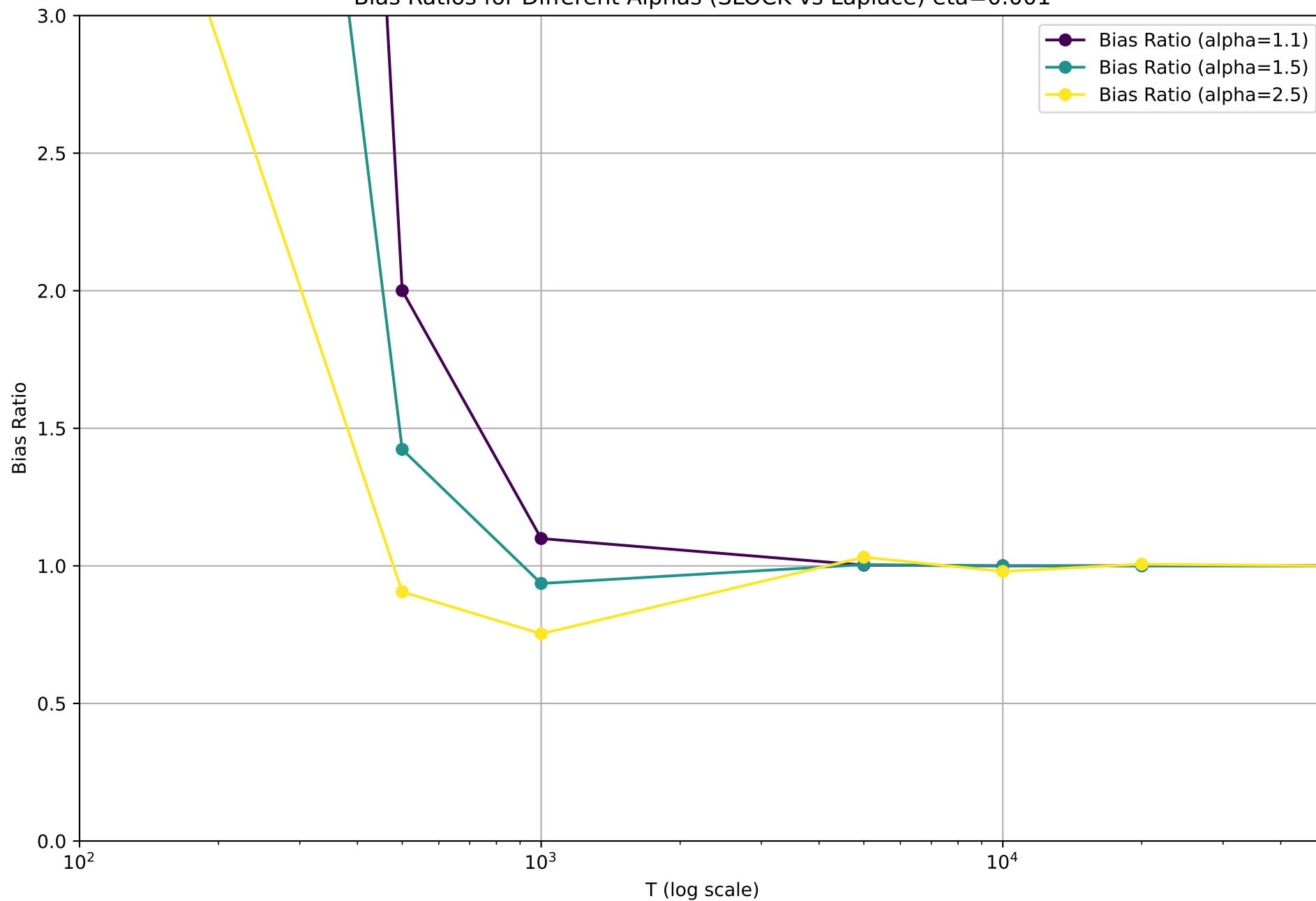
Bias Ratios for Different Alphas (SLOCK vs Laplace) \eta=0.001
