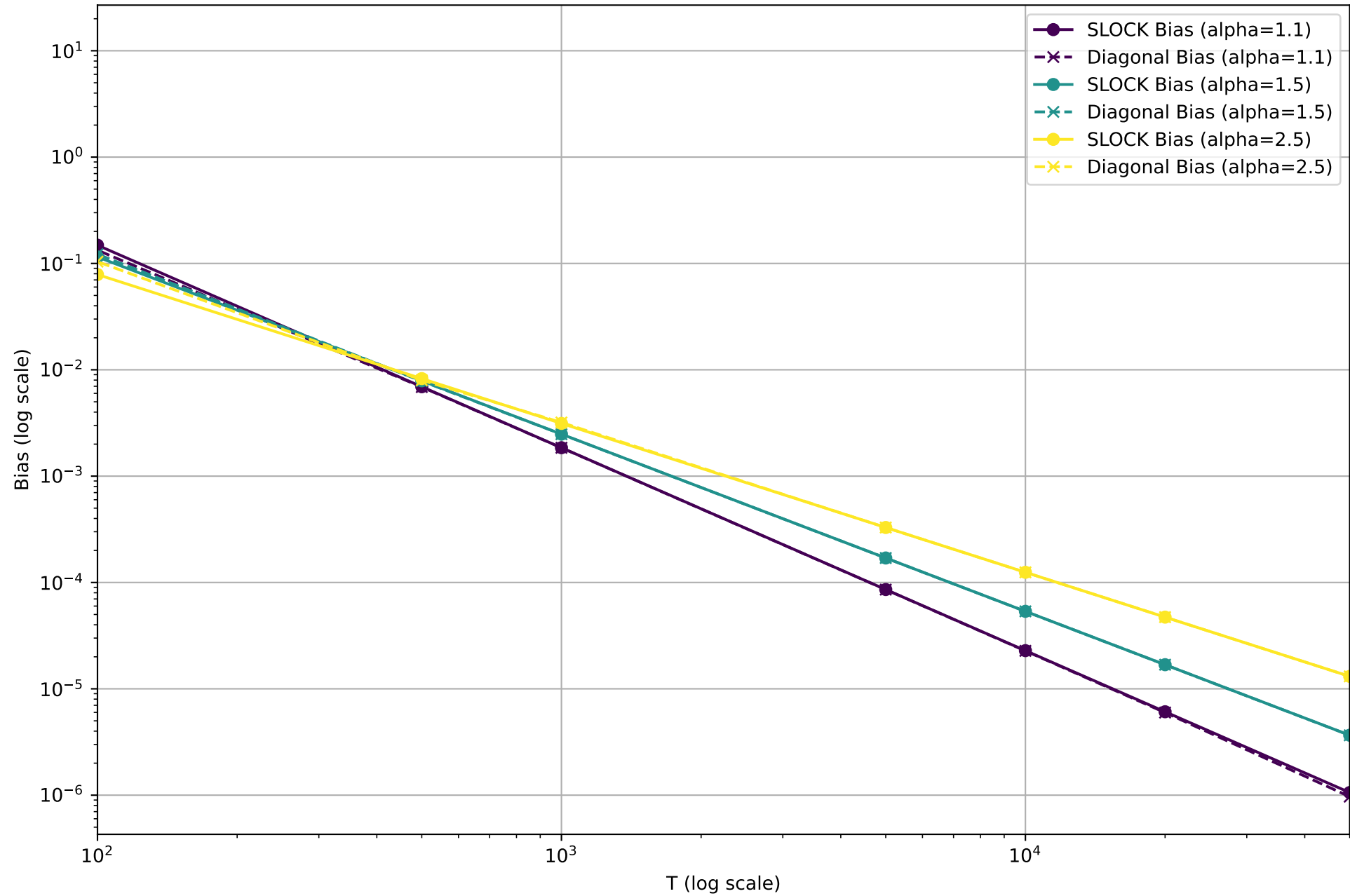
Bias Trajectories for Different Alphas (SLOCK vs Diagonal) \eta=0.01
