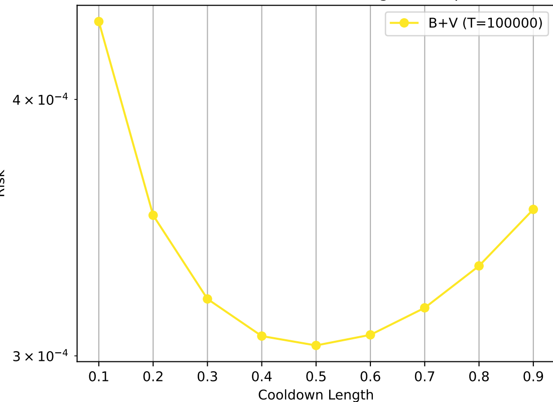
Risk for \eta=0.001 (SLOCK vs Diagonal), \alpha=2.5
