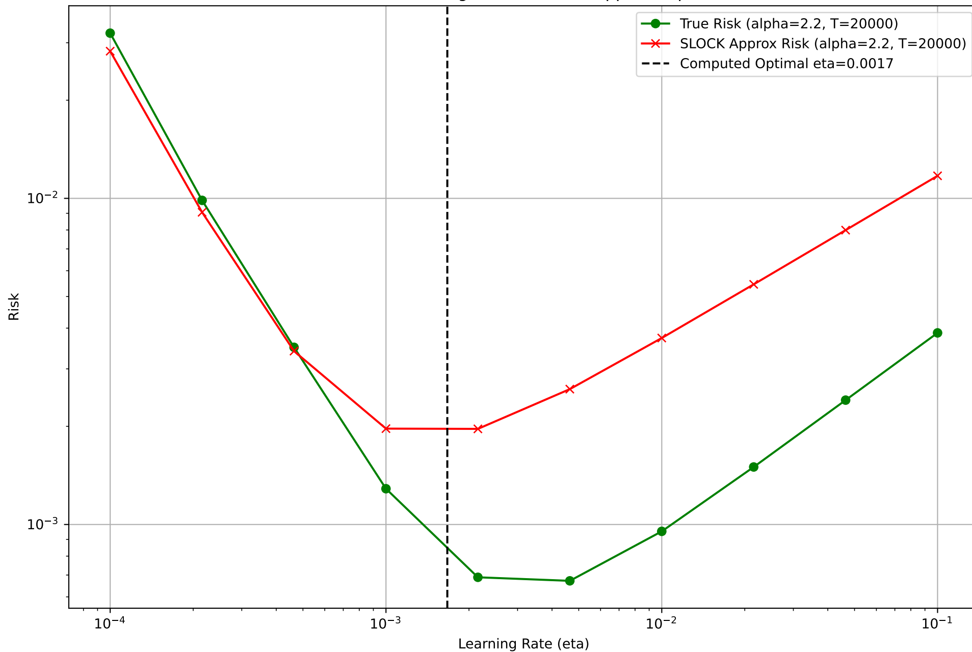
True Risk for Different Learning Rates (True vs Approx) \alpha=2.2 , T=20000
