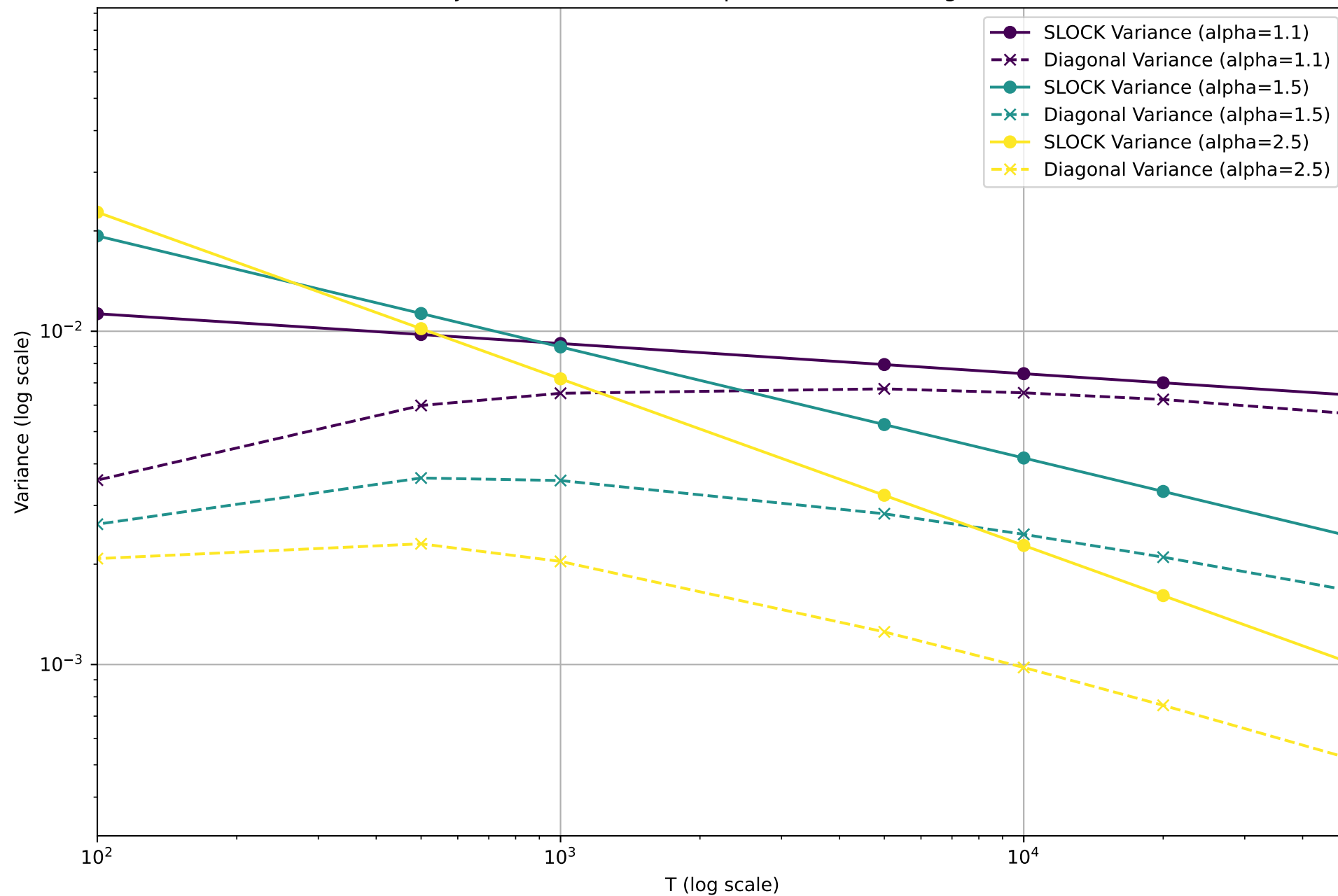
Variance Trajectories for Different Alphas (SLOCK vs Diagonal) \eta=0.01
