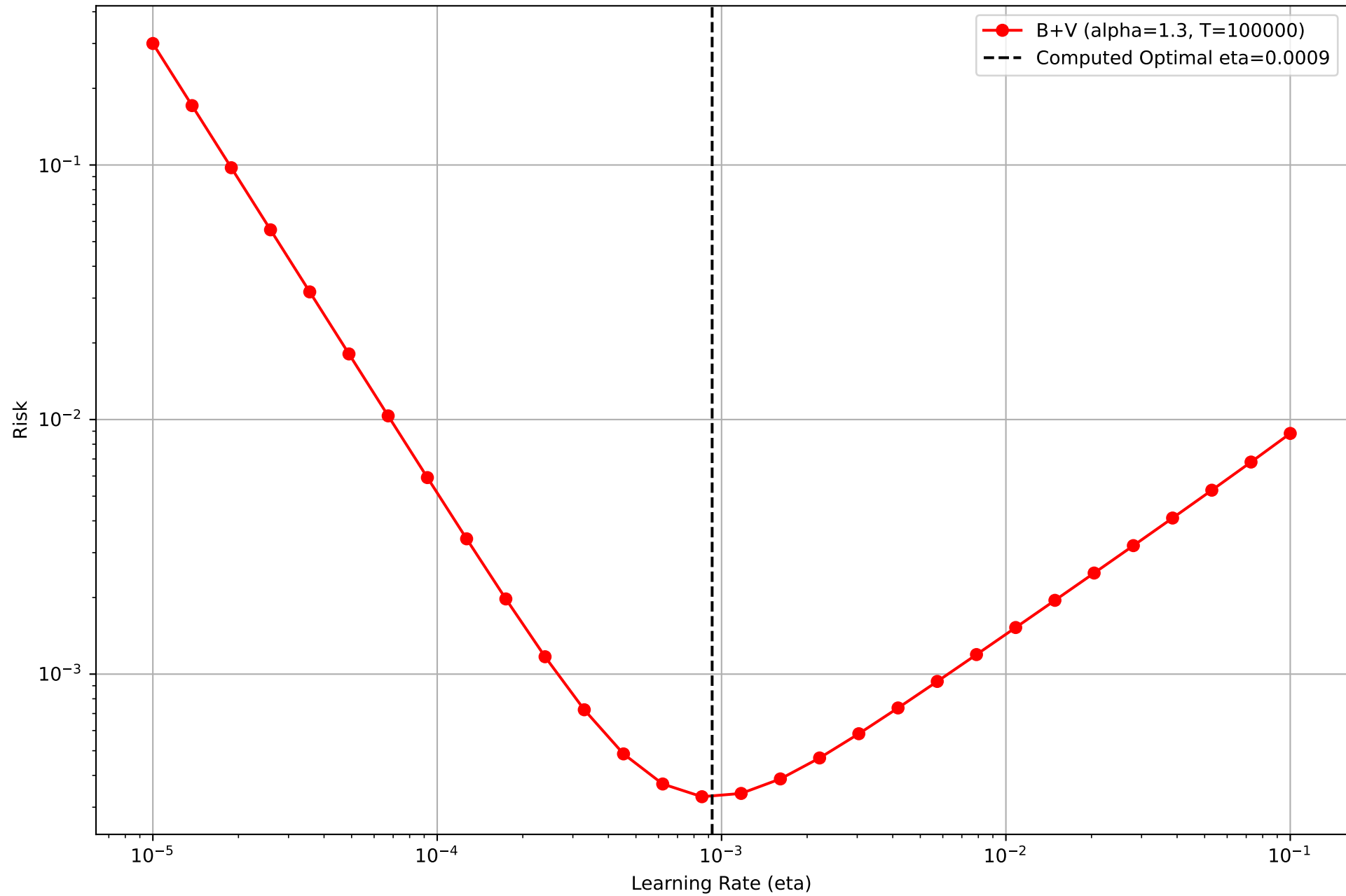
Risk for Different Learning Rates (True vs Approx) \alpha=1.3 , T=100000
