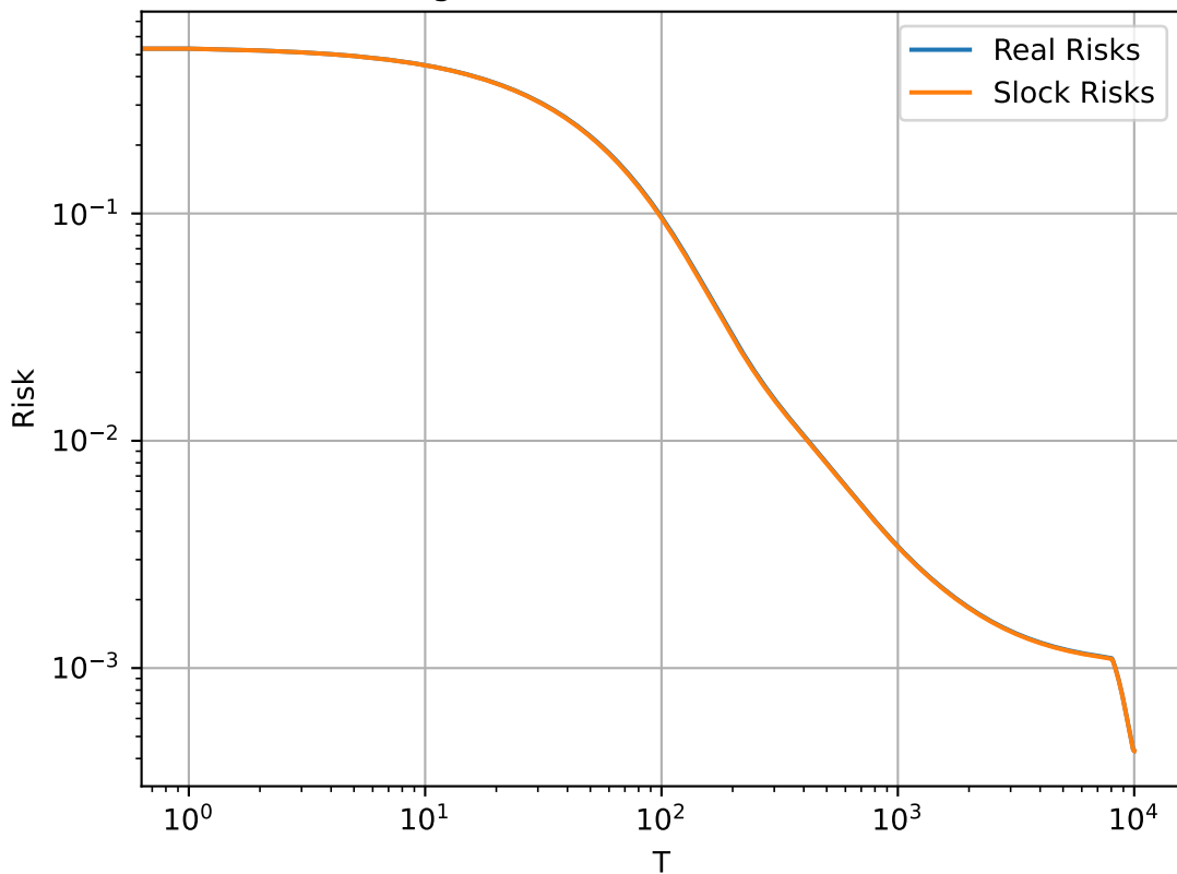
Comparison of Real Risks and Slock Risks for SGD with WSD schedule \sigma=0.5 , \beta=2 , T=10000
