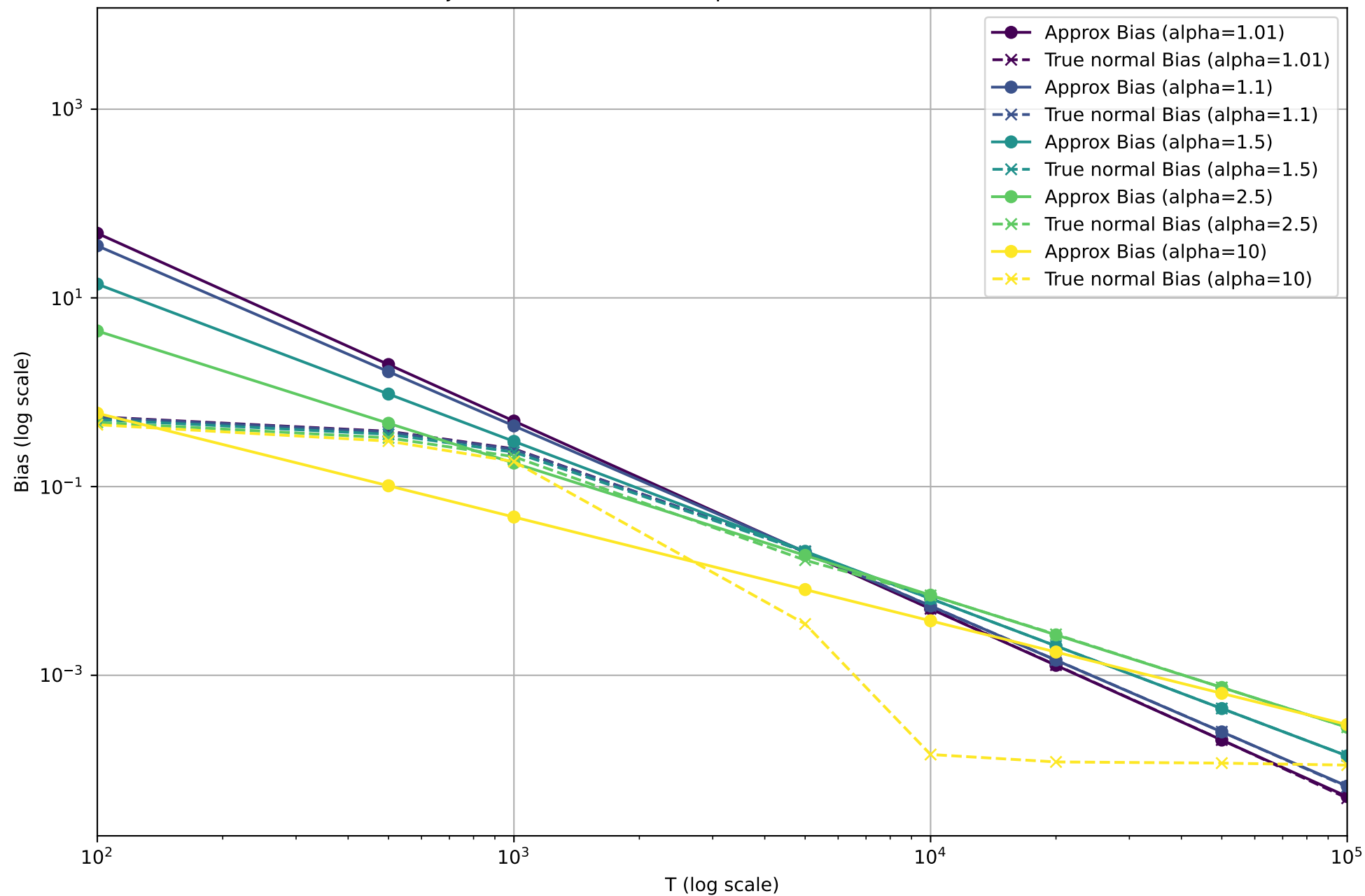
Bias Trajectories for Different Alphas (normal vs True) eta=0.001
