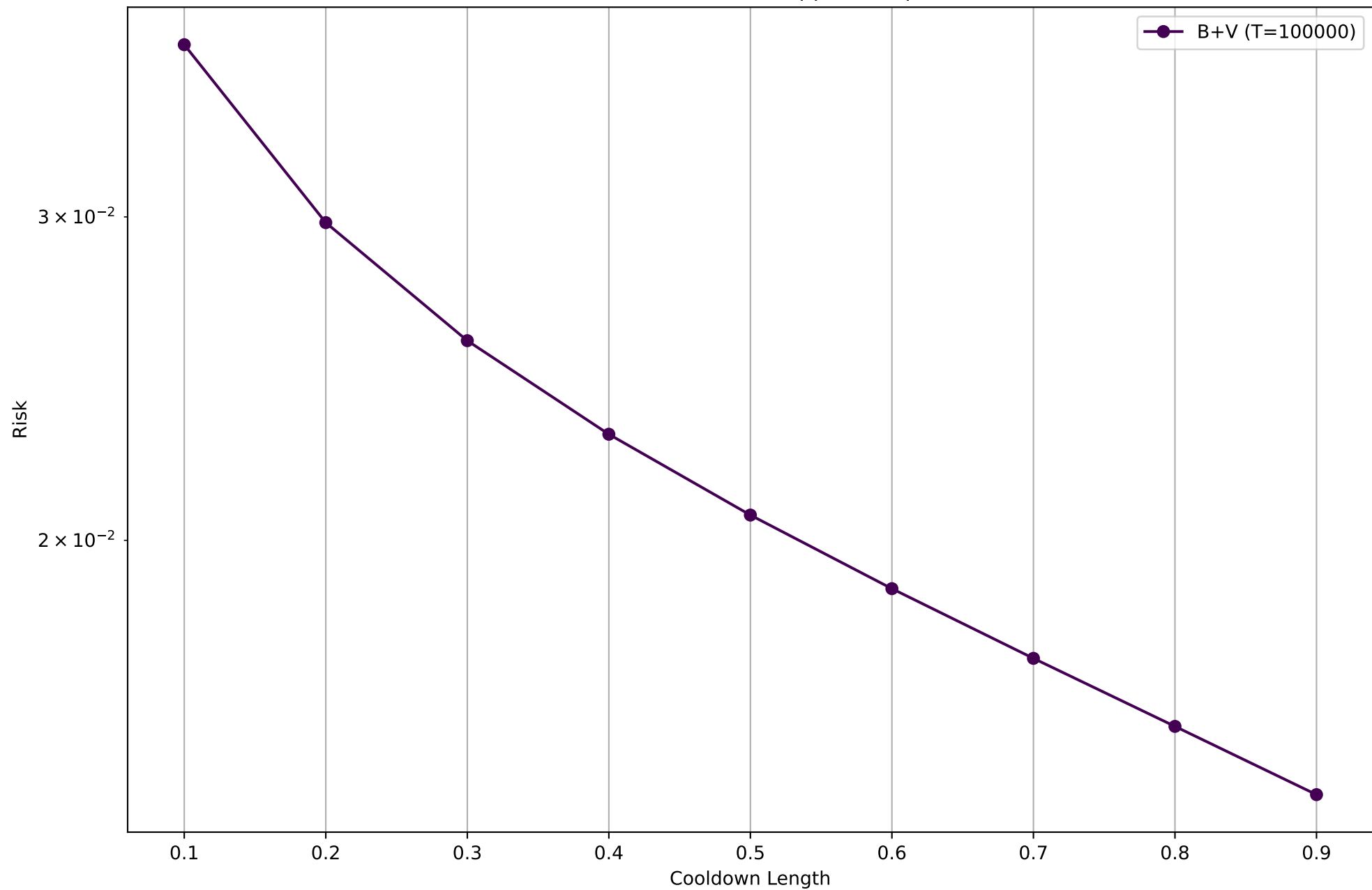
Risk for eta=0.1 (True vs Approx), alpha=1.2
