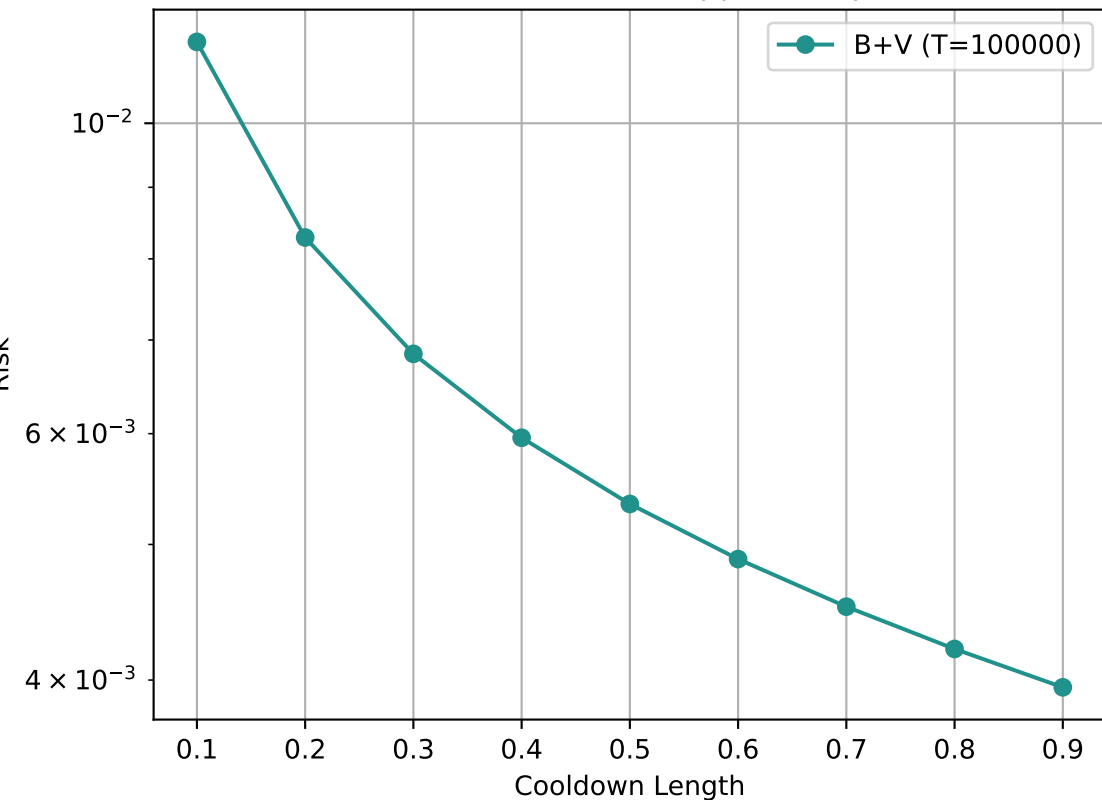
Risk for eta=0.1 (True vs Approx), alpha=1.8
