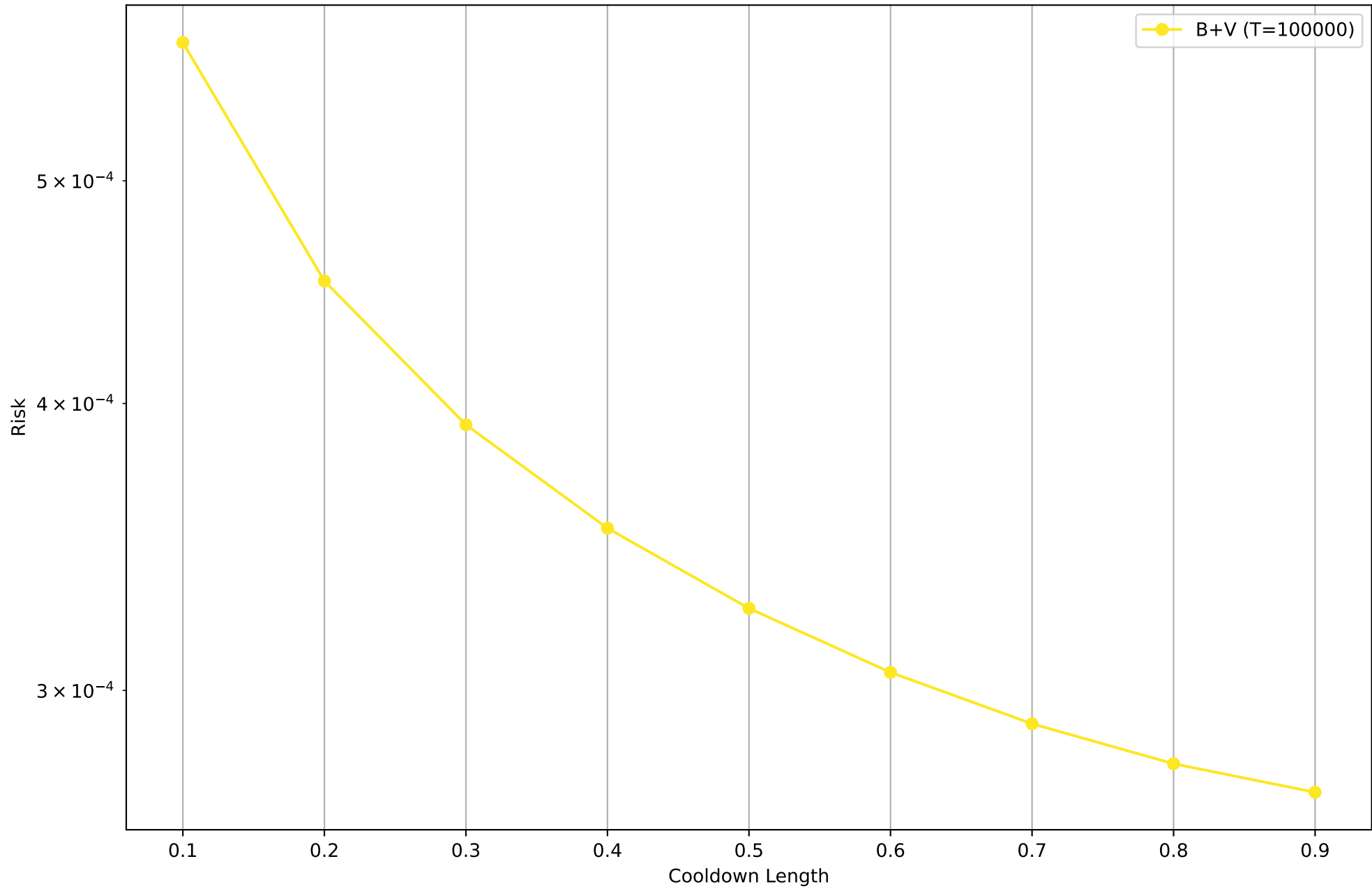
Risk for Different cooldown lengths (SLOCK vs Diagonal) eta=0.001, alpha=1.4
