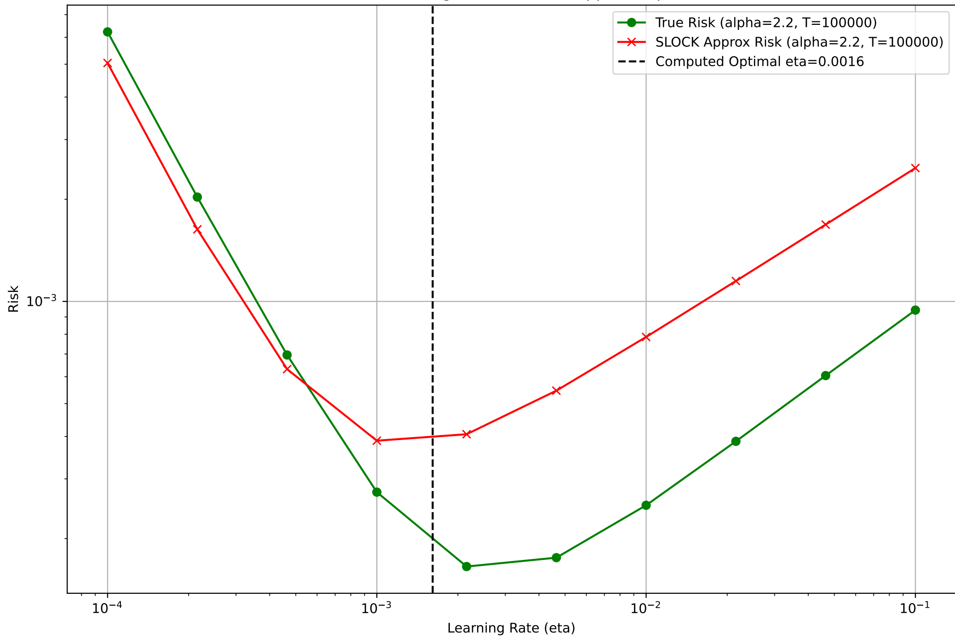
True Risk for Different Learning Rates (True vs Approx) \alpha=2.2 , T=100000
