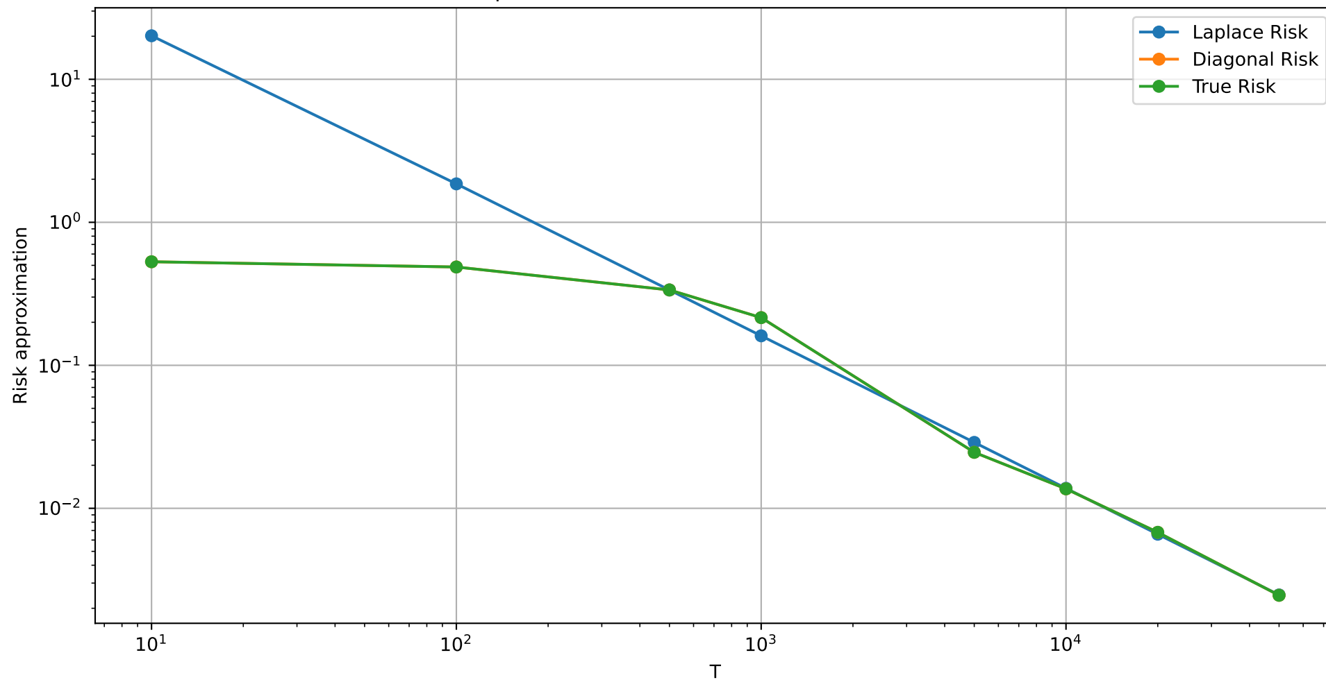
Total risk of Laplace approximation vs Diagonal approximation for linear schedule \alpha=3 , \beta=1.2 , T_{\max}=50000 , K=t/T=1
