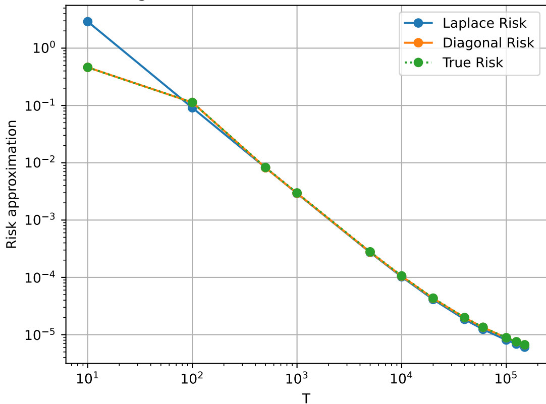
Total risk of Laplace approximation vs Diagonal approximation for wsd schedu sigma=0.1, beta=2, Tmax=150000, K=t/T=1
