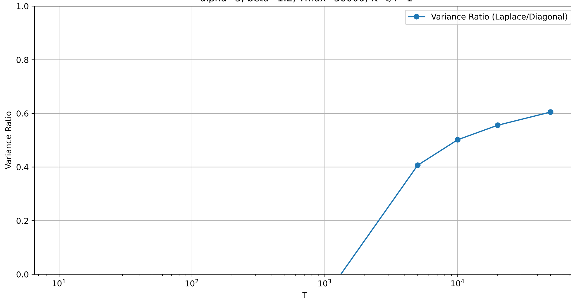
Variance Ratio of Laplace approximation to Diagonal approximation for linear schedule \alpha=3 , \beta=1.2 , T_{\max}=50000 , K=t/T=1
