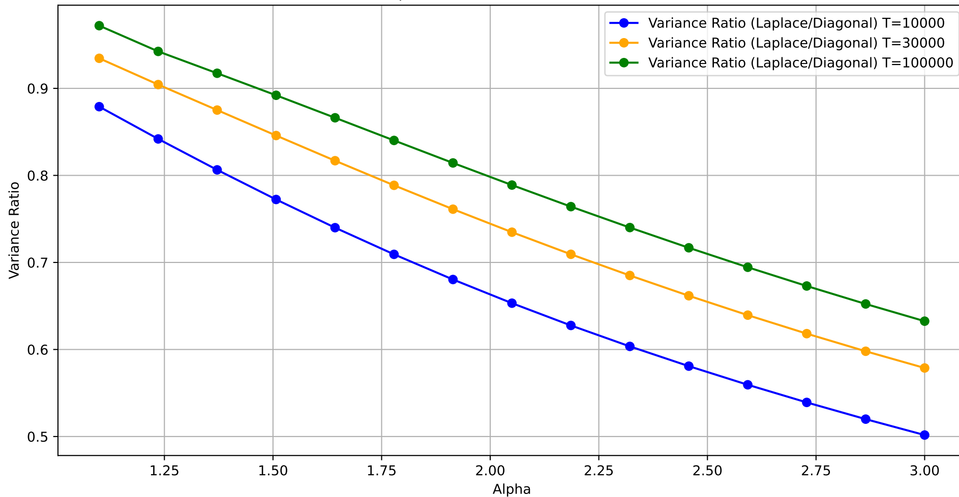
Variance Ratio of Laplace approximation to Diagonal approximation for linear schedule at K=1 for different alpha values, beta=1.2, Delta=1, dim=1000
