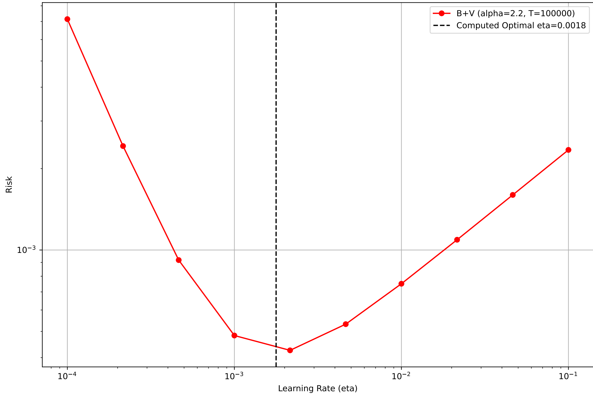
Risk for Different Learning Rates (True vs Approx) \alpha=2.2 , T=100000
