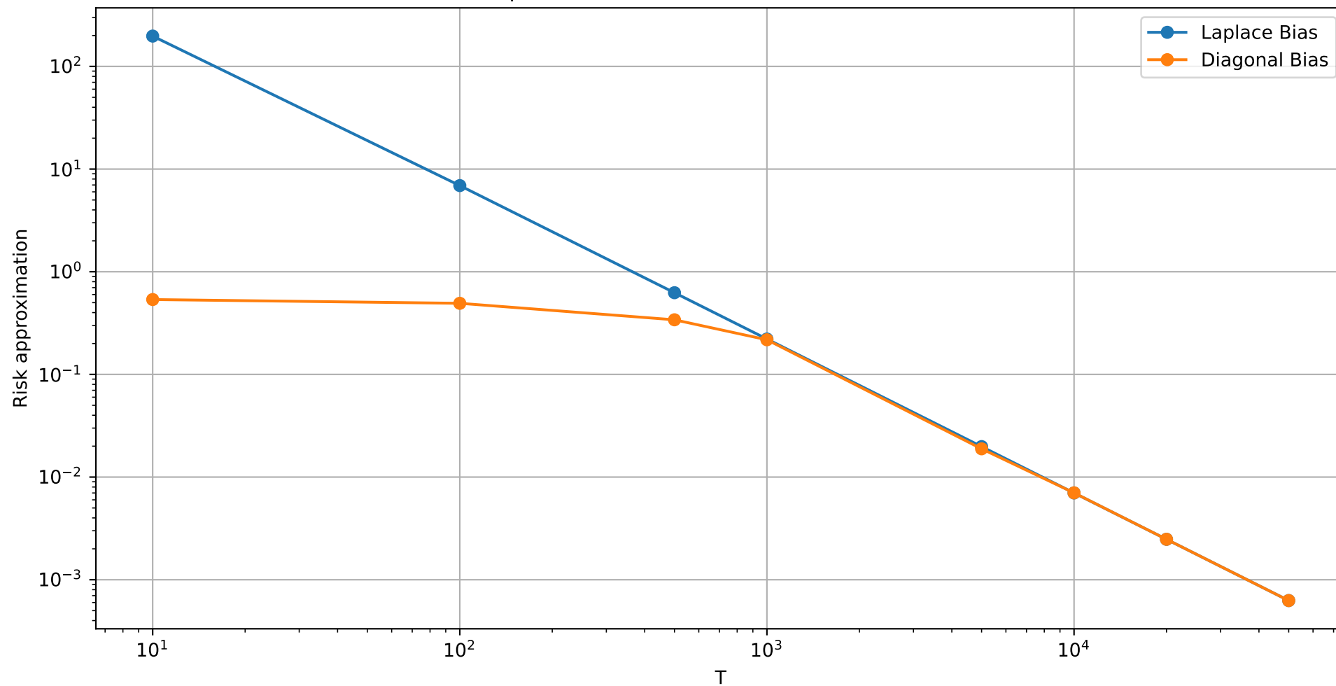
Bias components of Laplace approximation vs Diagonal approximation for linear schedule \alpha=2 , \beta=2 , T_{\max}=50000 , K=t/T=1
