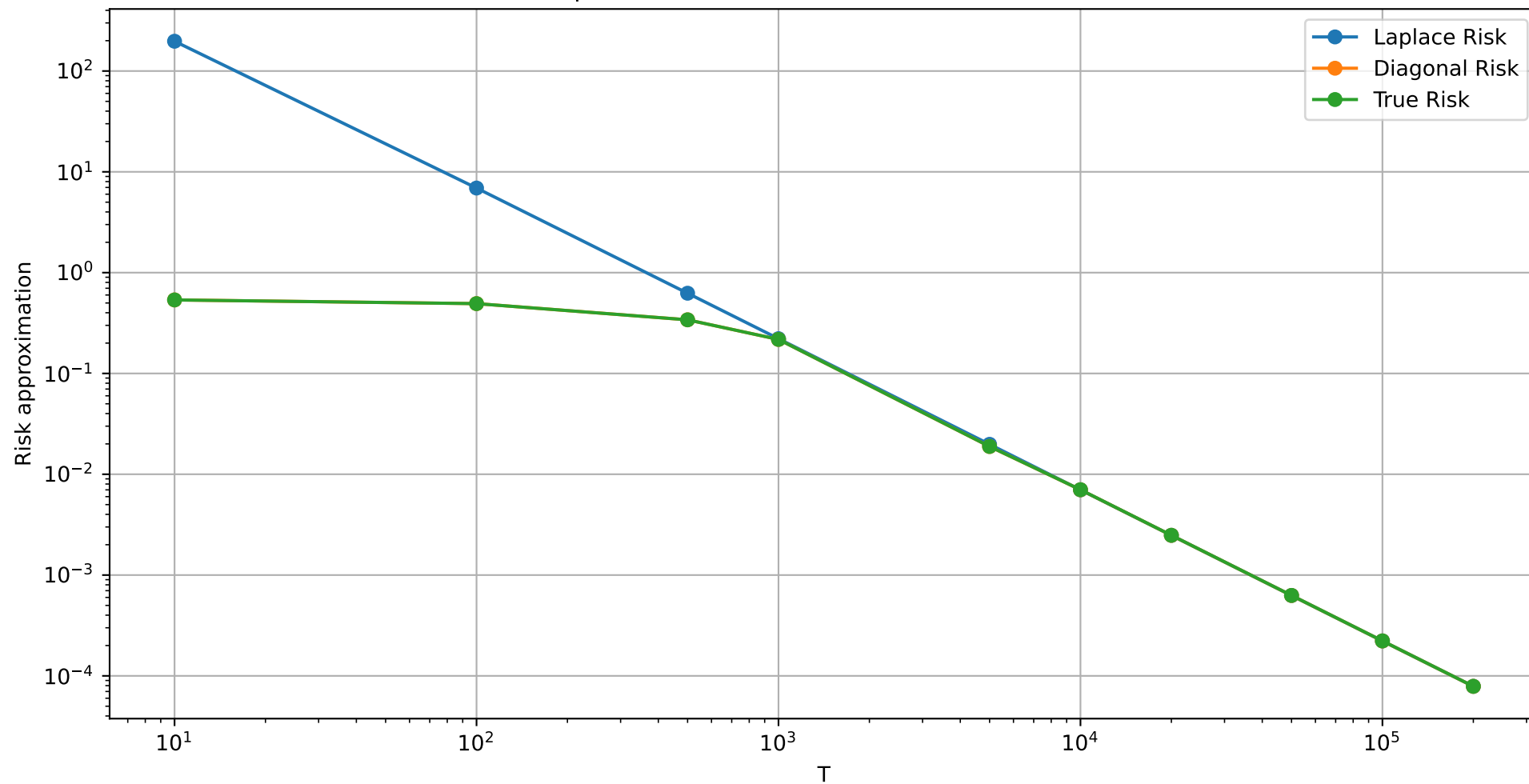
Total risk of Laplace approximation vs Diagonal approximation for linear schedule \alpha=2 , \beta=2 , T_{\max}=200000 , K=t/T=1
