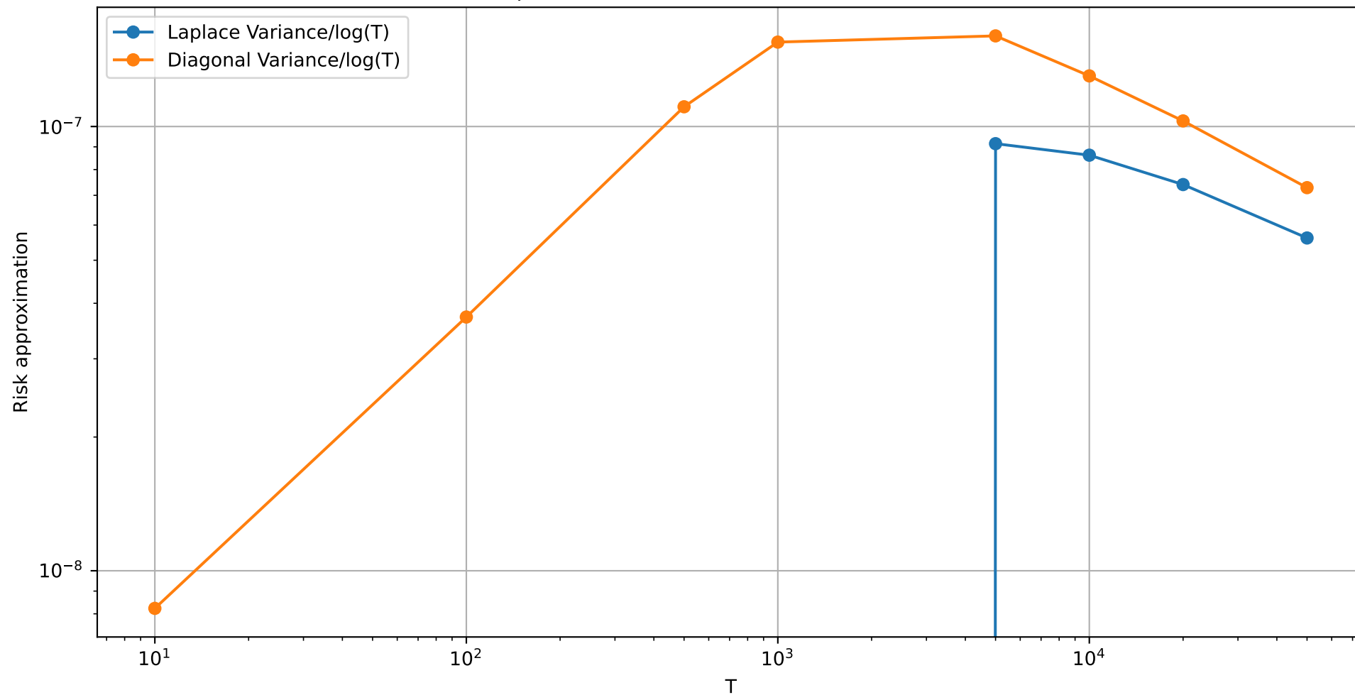
Variance components of Laplace approximation vs Diagonal approximation for linear schedule ( 1/\log(T) ) \alpha=2, \beta=2, T_{\max}=50000, K=t/T=1
