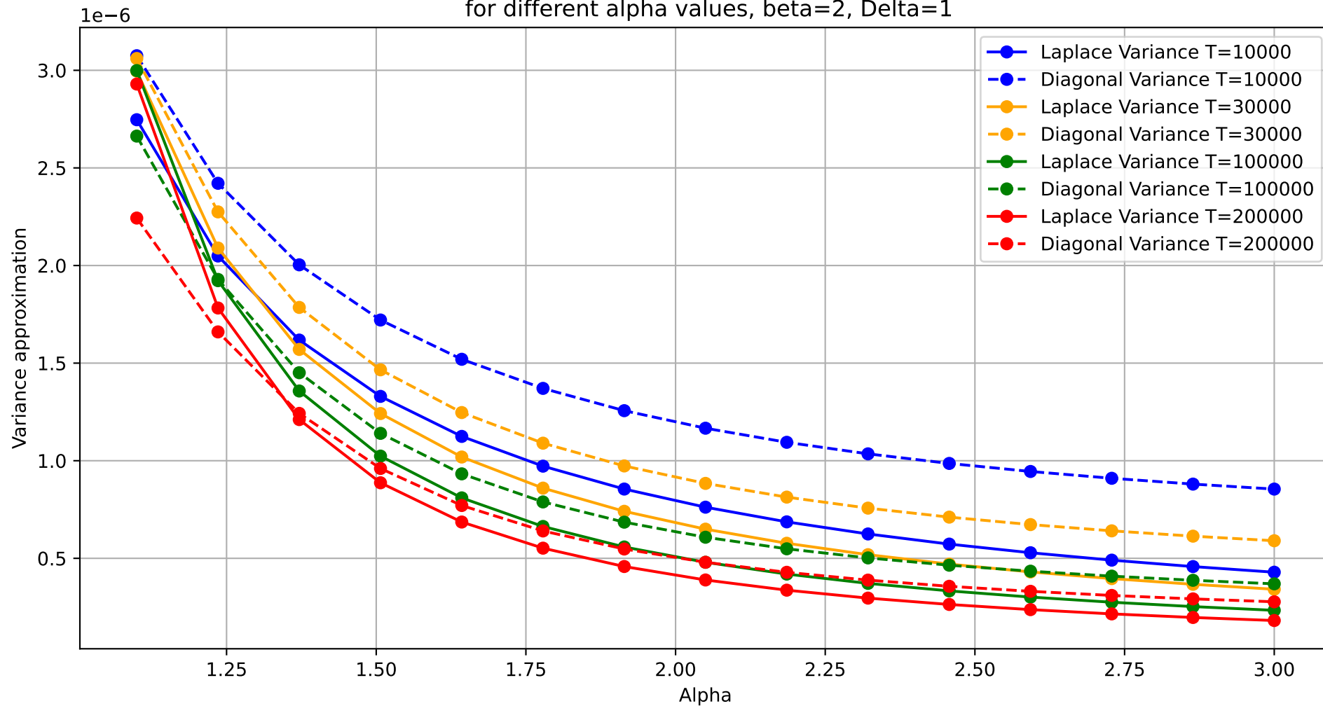
Variance of Laplace approximation vs Diagonal approximation for linear schedule at K=1 for different alpha values, beta=2, Delta=1
